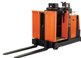
OME100 with auxiliary lift and OME100W walk-through version • Chassis width 970 mm • Maximum capacity 1000 kg • Picking heights to 3.35 m • Cabin widths 1000 mm, 1200 mm, 1400 mm
